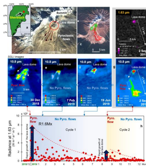
Fig. 3. Pyroclastic flows / 2018-2019 Sheveluch, Russia
