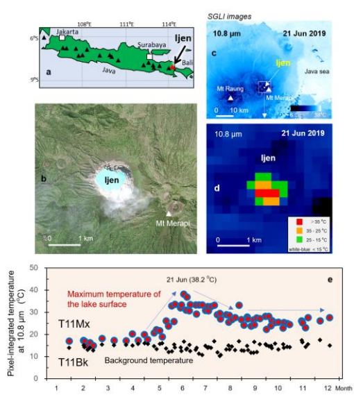
Fig. 5. Active crater lake / 2019 Ijen, Indonesia
