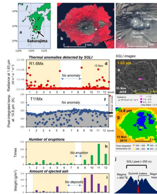
Fig. 4. Small-scale Vulcanian eruptions / Sakurajima, Japan
