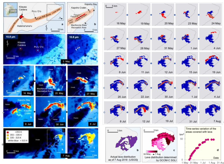
Fig. 2. Large-scale lava effusion / 2018 Kilauea, Hawaii
