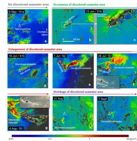
Fig. 6. Large-scale discolored seawater areas observed in the 2019-2020 Nishinoshima eruption
